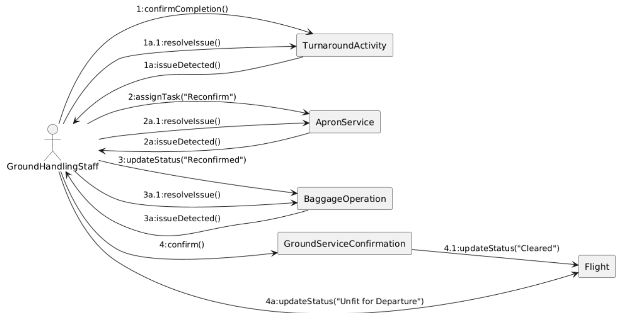
UC-27 Final Confirmation - Collaboration Diagram
