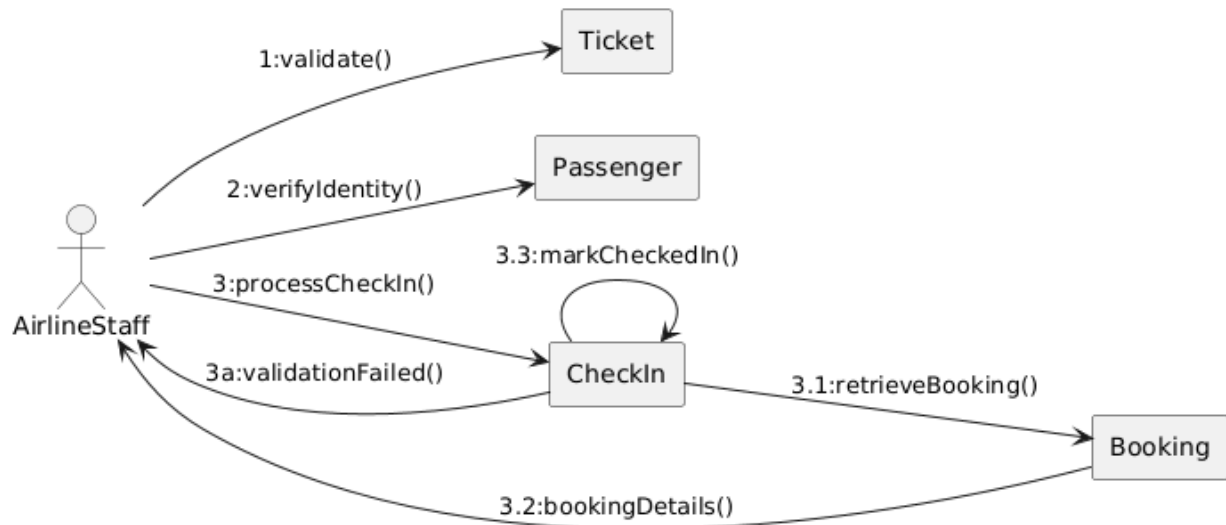
UC-28 Passenger Check-in - Collaboration Diagram
